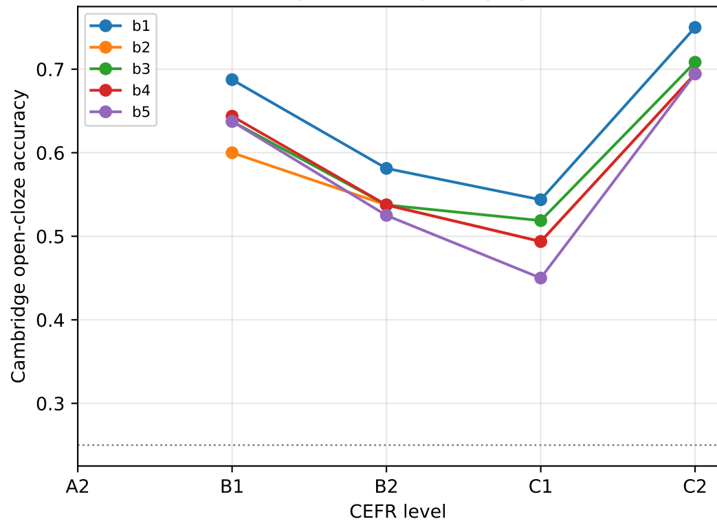
§4.1 Cambridge cloze trajectory by curriculum
